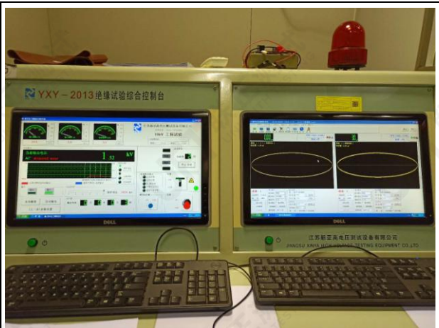
测试后局部放电确认 Partial discharge confirmation after test
