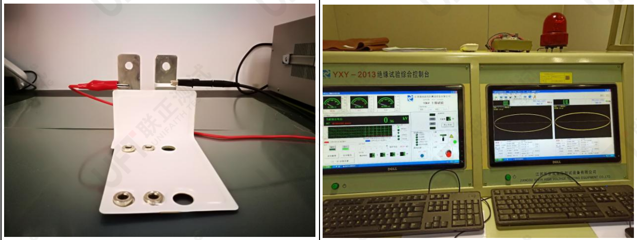
测试后局部放电确认 Partial discharge confirmation after test
